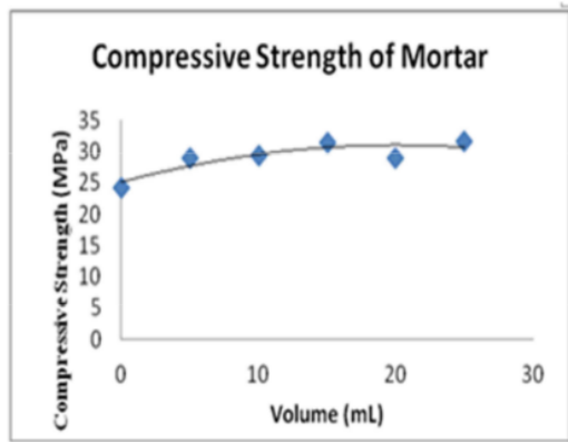
Figure 5. The graphic of the compressive strength vs the silver nanoparticle solution of the mortar.
