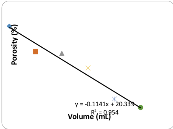
Figure 4. The graphic of the porosity vs silver nanoparticle volume of the mortar samples.
