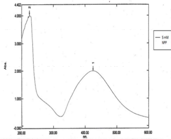
Figure 3. The result of 5 mM silver nanoparticle test using spectroscopy Uv-Vis.
